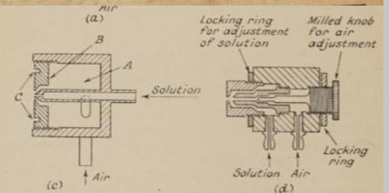
FIG. 19.—Atomizers for spray tests.
